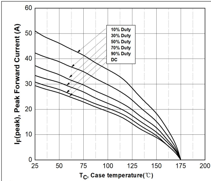
Figure 3. Current Derating
